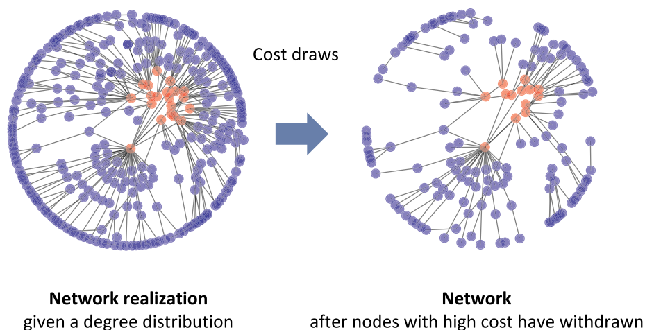
Figure 1. (Color online) An Illustration of the Timing of our Model in One Market
