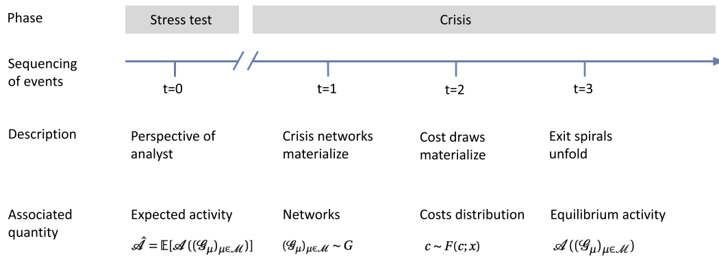
Figure 2. (Color online) Stress Testing and Crisis Timeline
