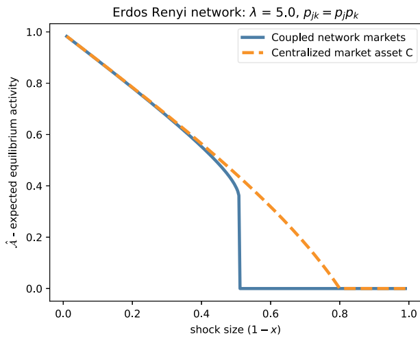
Figure 4. (Color online) Erdős-Rényi Network Example
