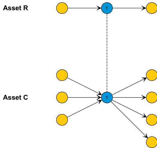
Figure 3. (Color online) Illustrative Example of a Fragile Connector
