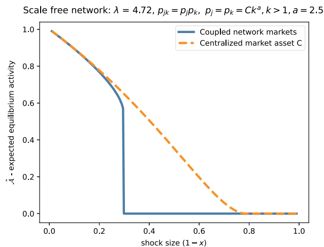
Figure 5. (Color online) Scale-Free Network Example
